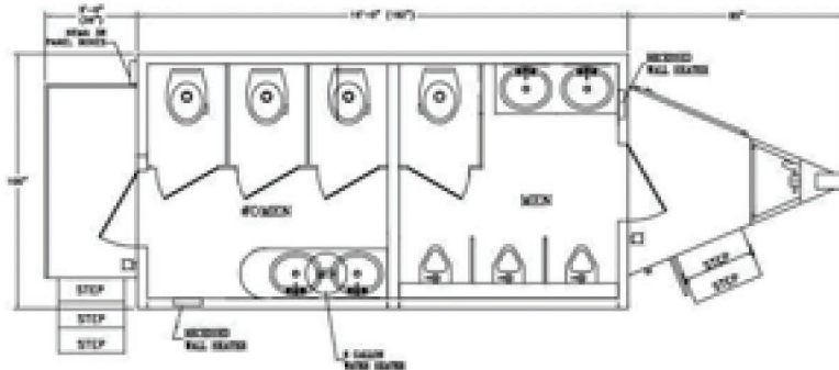
16 Foot Newport 1600 Series floor plan
